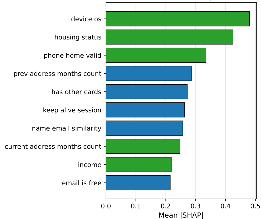
LGBM --- SHAP top-10
