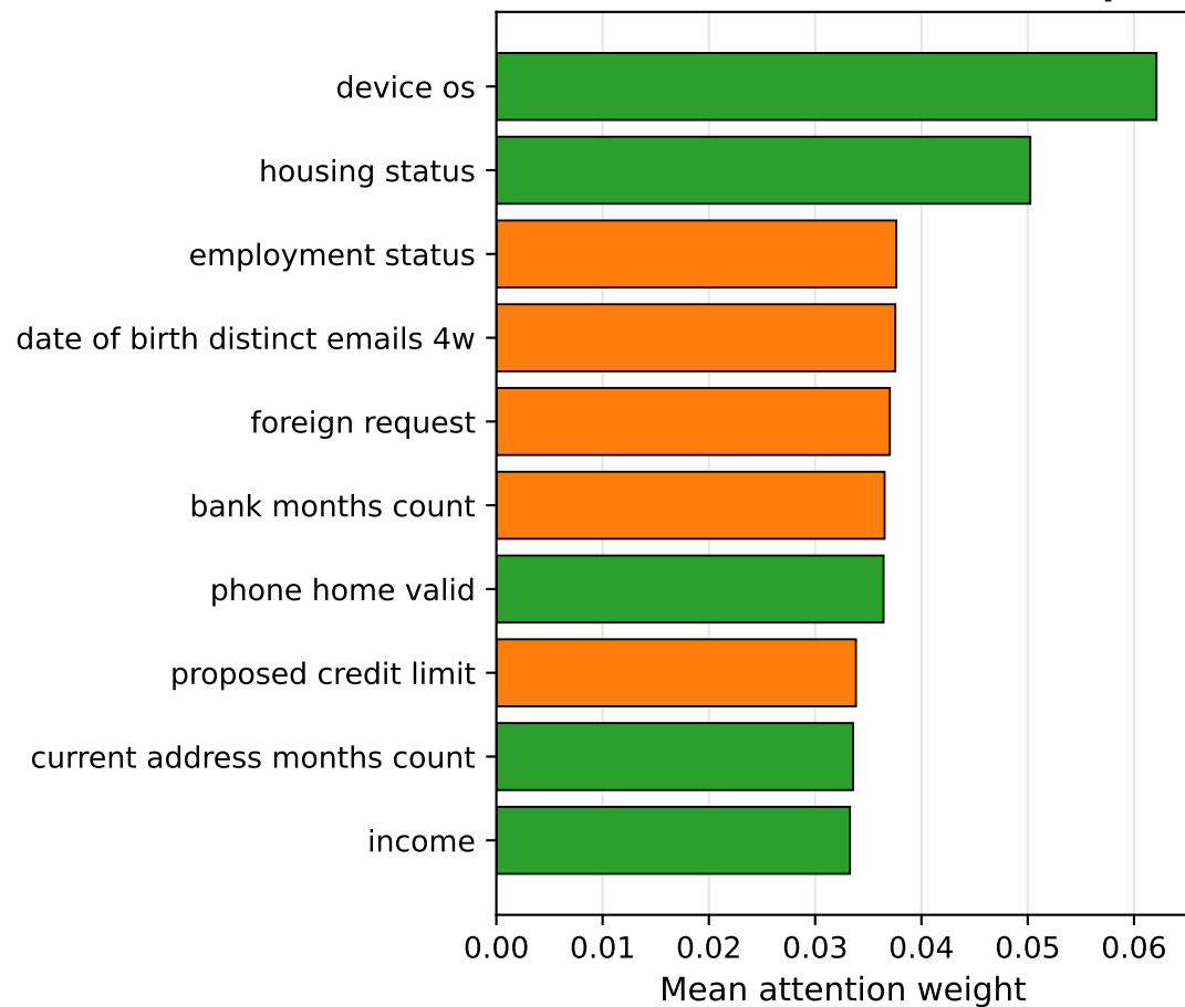
FT-Transformer --- Attention top-10
